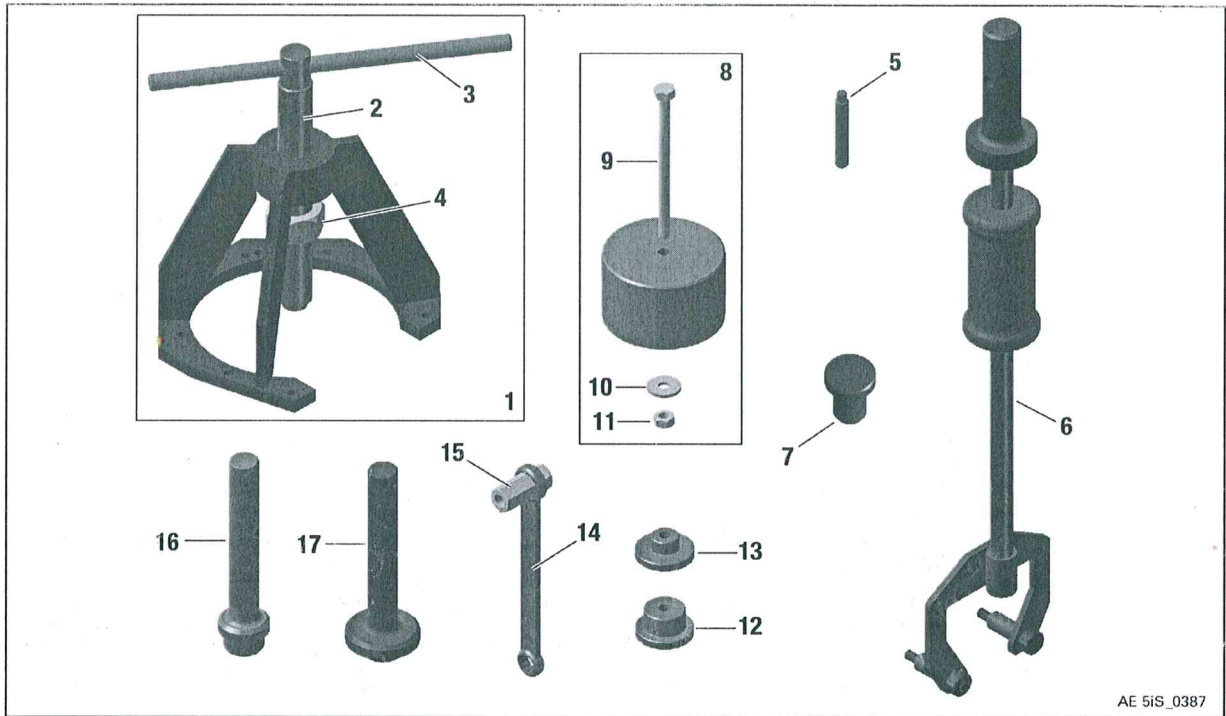
Figure 1.4: Repair tools
